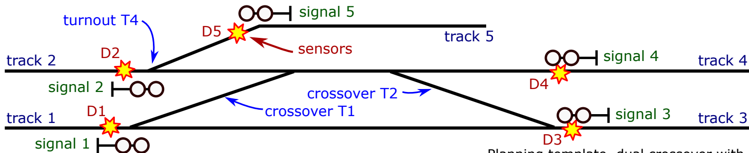
Planning template, dual crossover with narrow-side branch from track 2. Azatrax, (c) 2026
